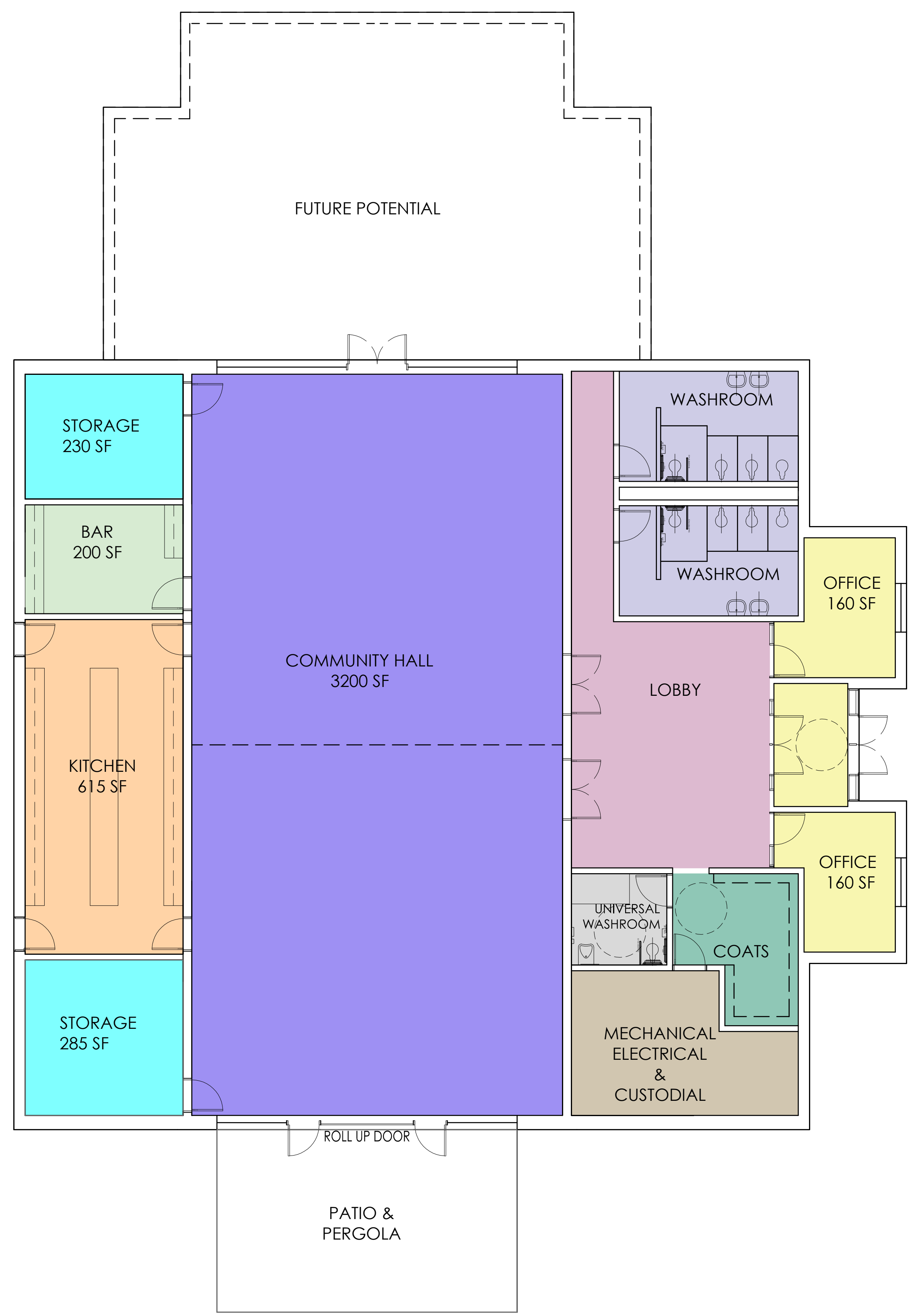
GROSS AREA 7,565 SQ FT SCHEMATIC FLOOR PLAN 0 1 2 5m
