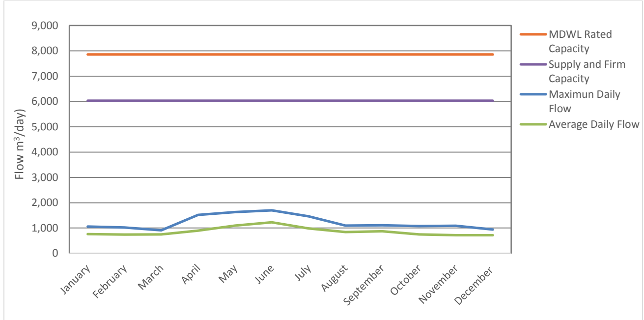
Figure 1 - 2023 Average vs Maximum Daily Flow Rates
