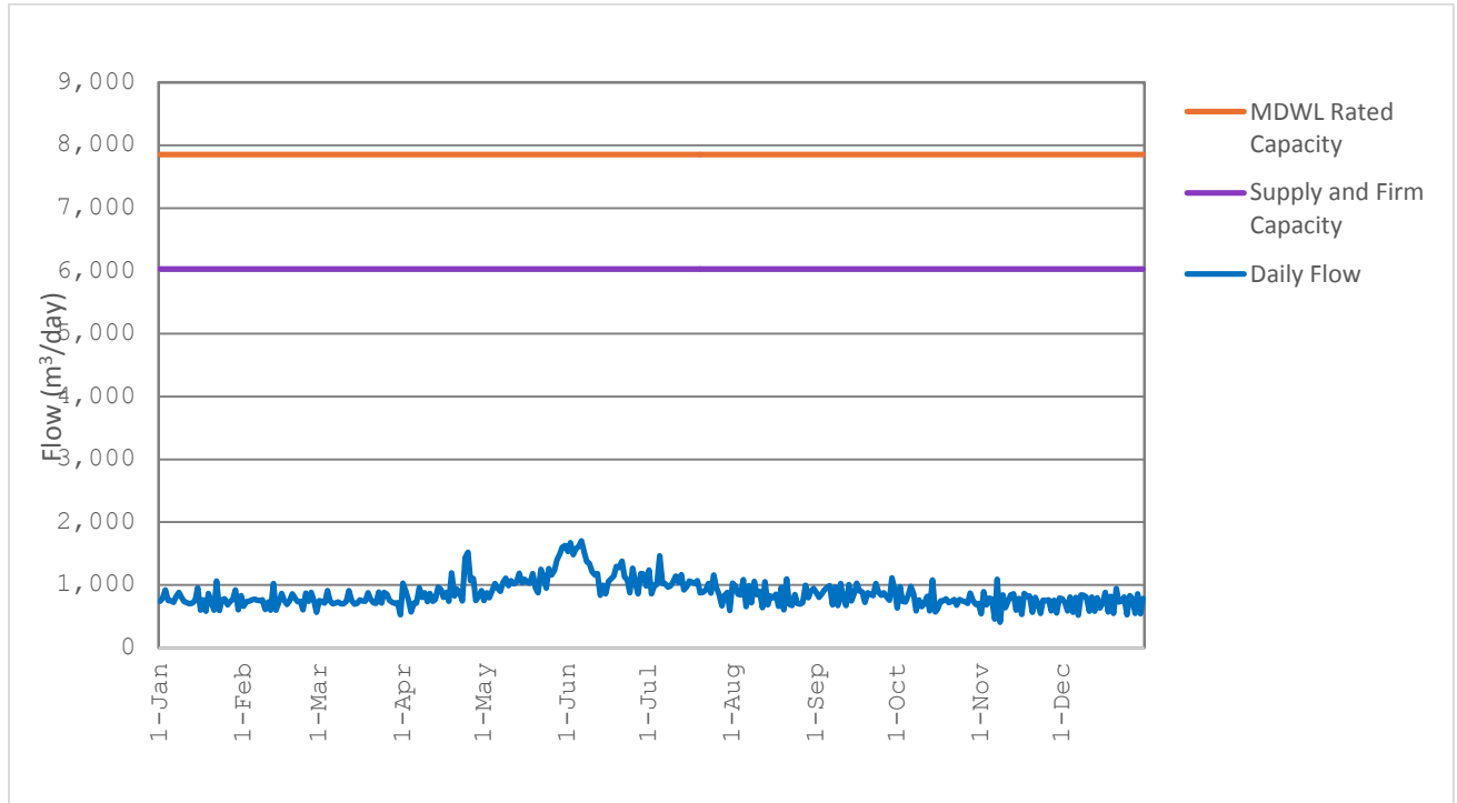
Figure 2 – 2023 Daily Flow Rates
